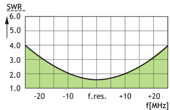
Typical VSWR curve
